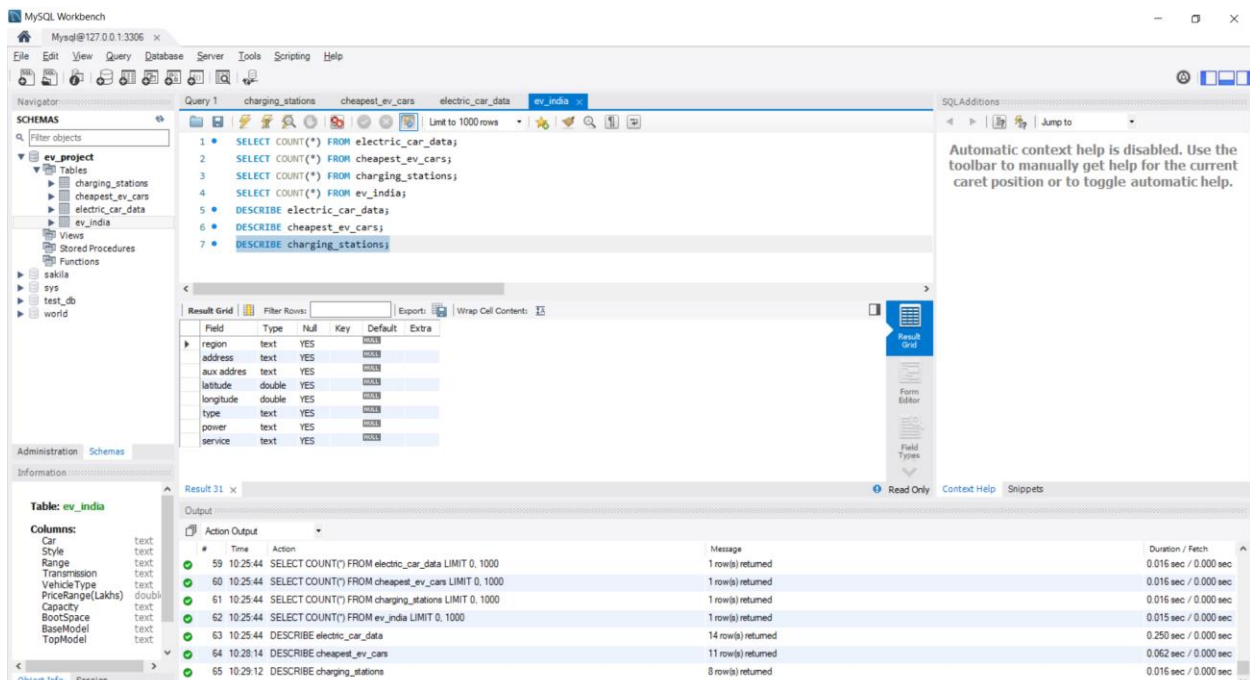
Figure 12.1: Structure of the Charging Stations Table Using the DESCRIBE Command
